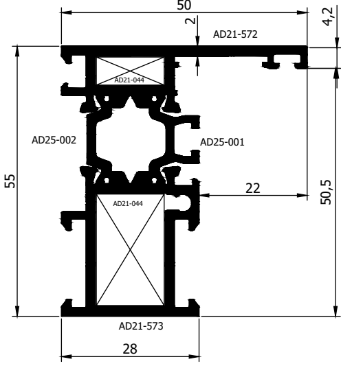
AD 21 - 056 ( 1,343 Kg/m )
