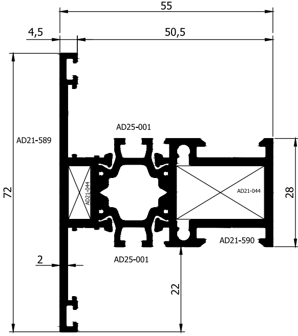
AD 21 - 066 ( 1,512 Kg/m )
