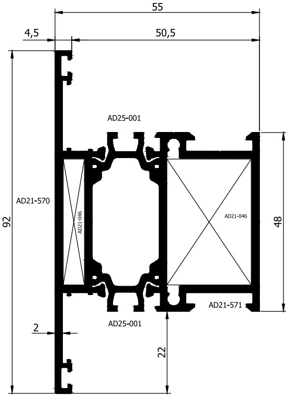
AD 21 - 055 ( 1,936 Kg/m )
