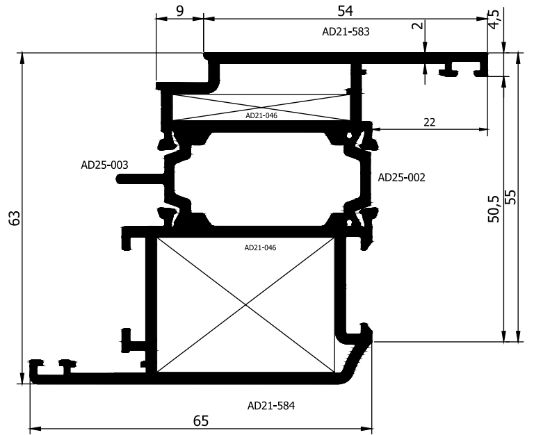
AD 21 - 063 ( 1,920 Kg/m )
