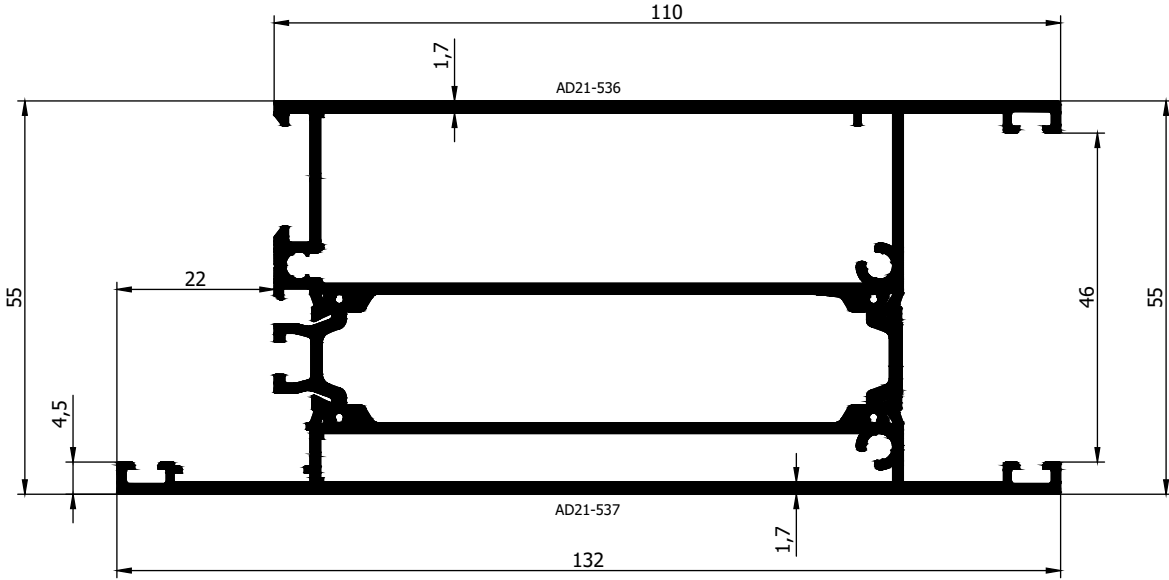
AD 21 - 020 ( 2,520 Kg/m )
