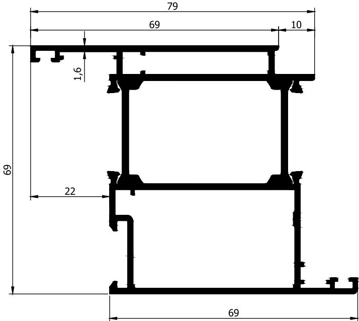
AD32-053 1,759 Kg/m
