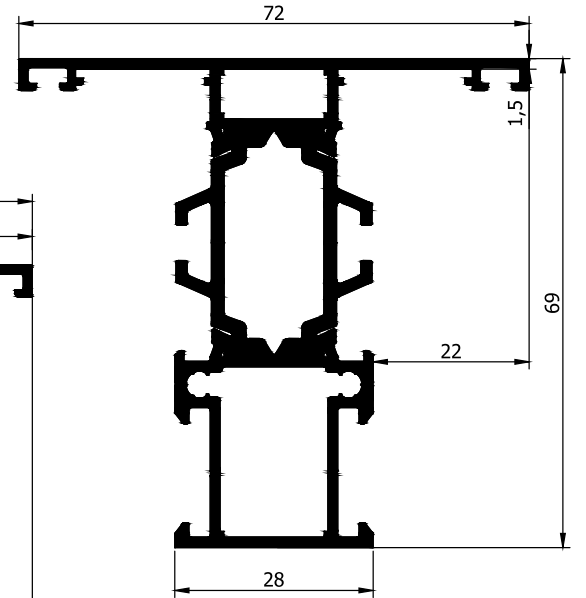
AD32-015 1,389 Kg/m
