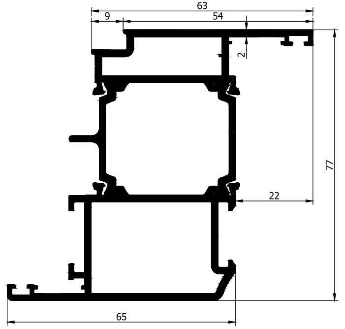
AD32-042 1,995 Kg/m
