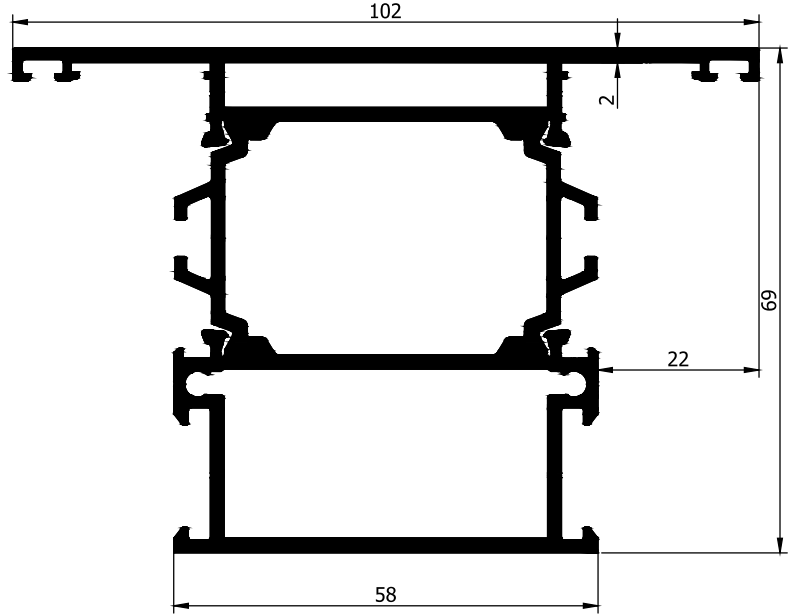
AD32-047 2,240 Kg/m
