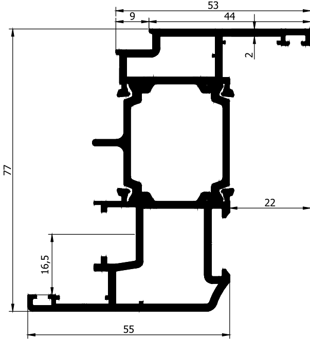
AD32-041 1,795 Kg/m
