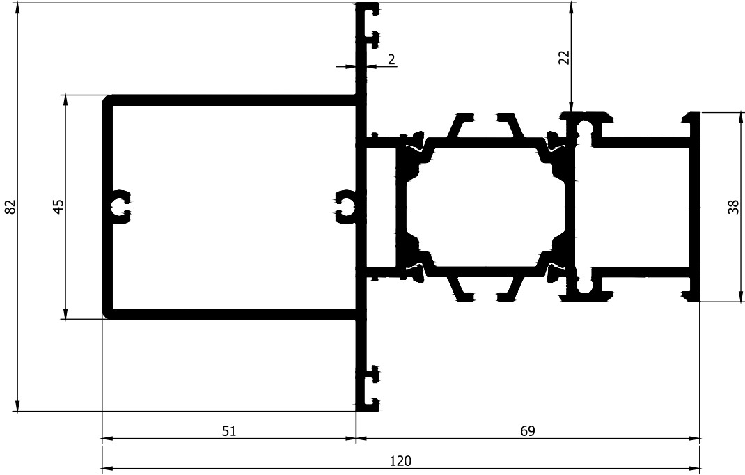
AD32-050 2,661 Kg/m
