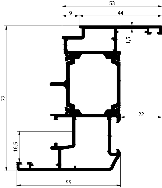
AD32-009 1,529 Kg/m
