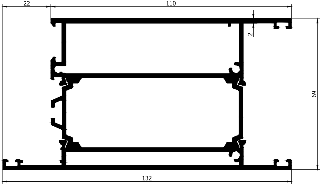
AD32-049 2,995 Kg/m
