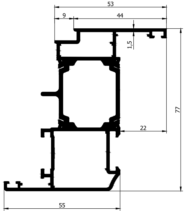
AD32-008 1,509 Kg/m
