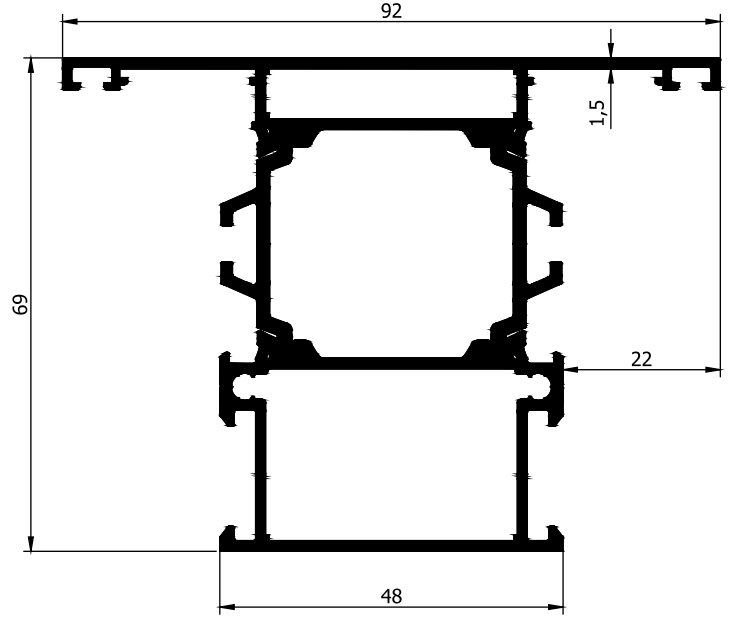
AD32-017 1,715 Kg/m
