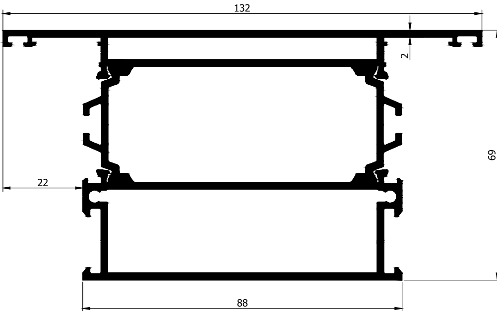
AD32-048 2,875 Kg/m
