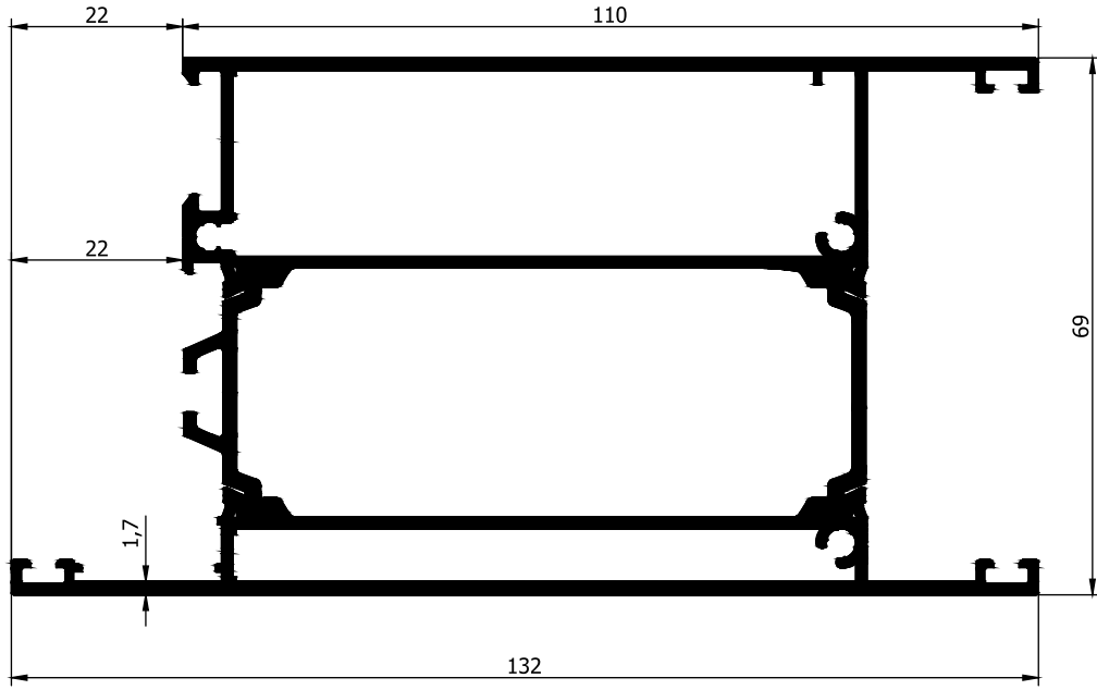
AD32-020 2,603 Kg/m
