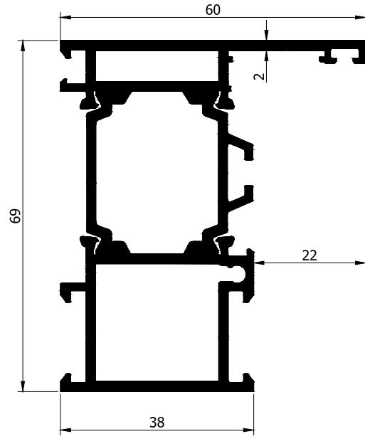
AD32-036 1,643 Kg/m
