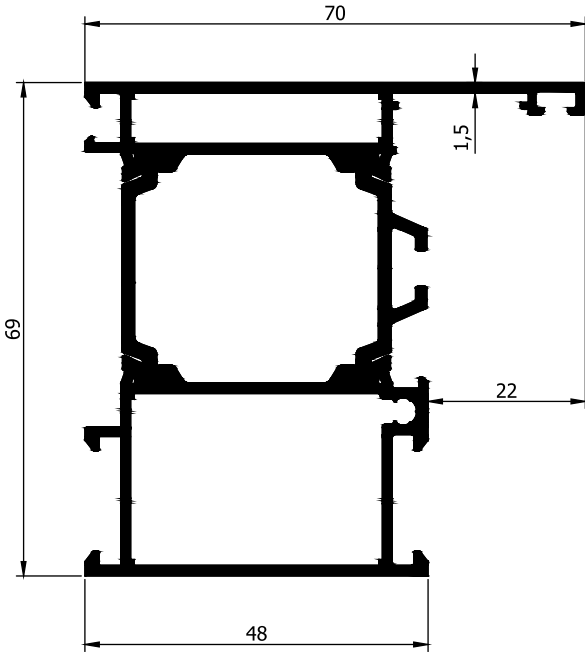
AD32-003 1,559 Kg/m
