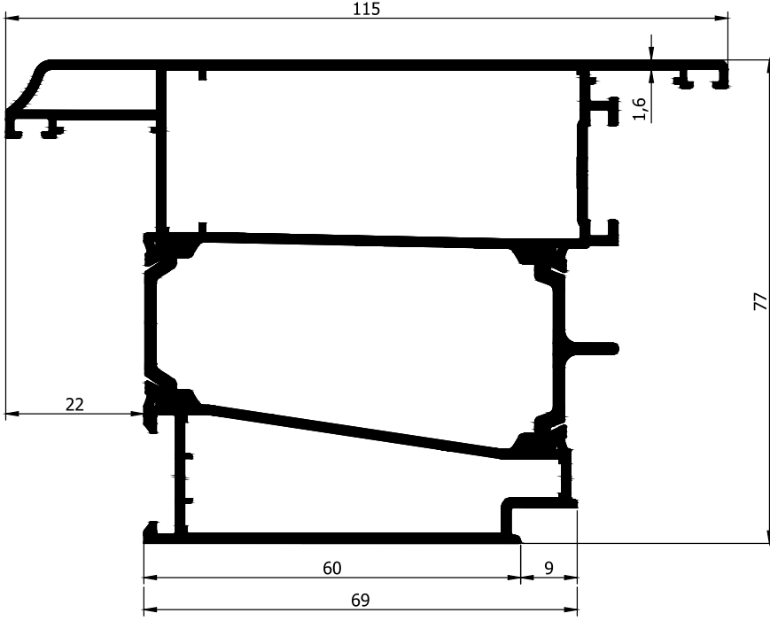
AD32-014 2,308 Kg/m
