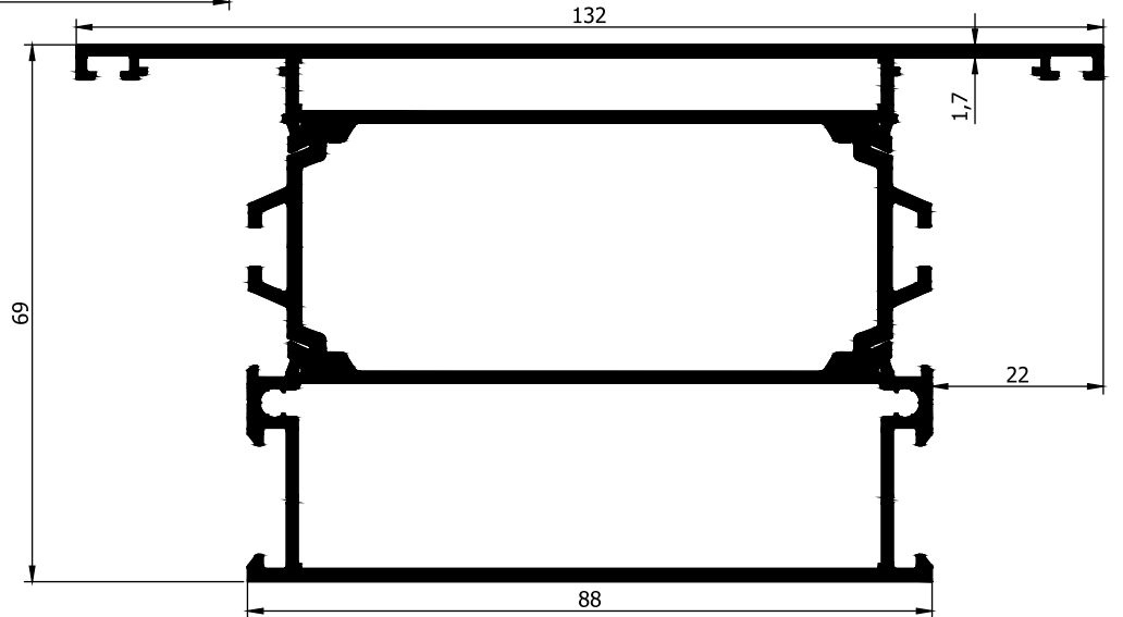
AD32-019 2,485 Kg/m
