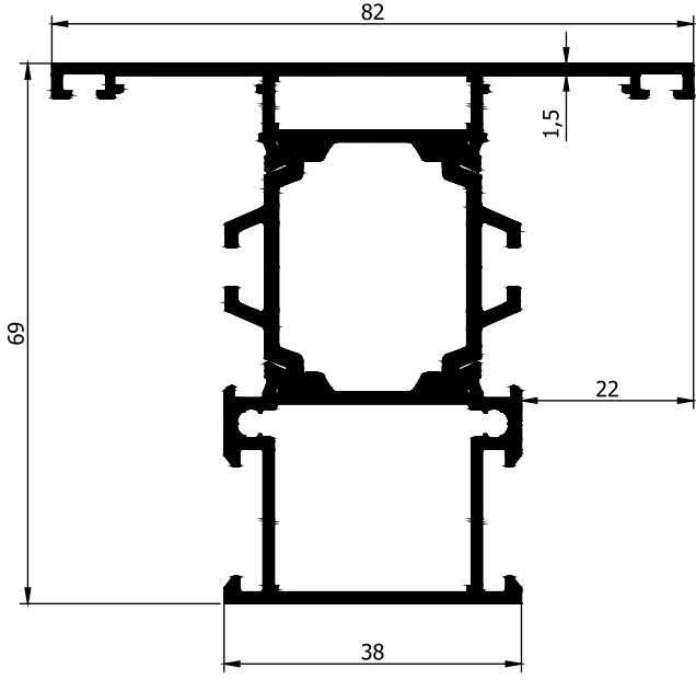
AD32-016 1,551 Kg/m
