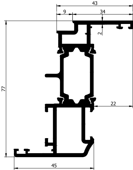
AD32-040 1,575 Kg/m
