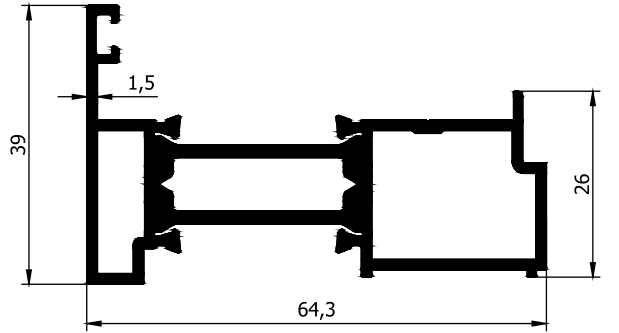
AD32-057 1,005 Kg/m
