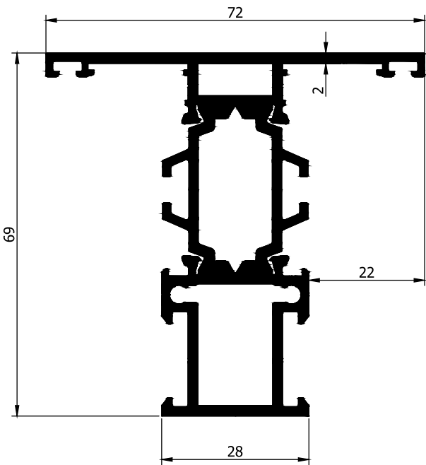
AD32-045 1,606 Kg/m
