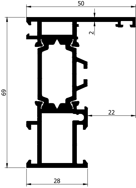
AD32-035 1,428 Kg/m
