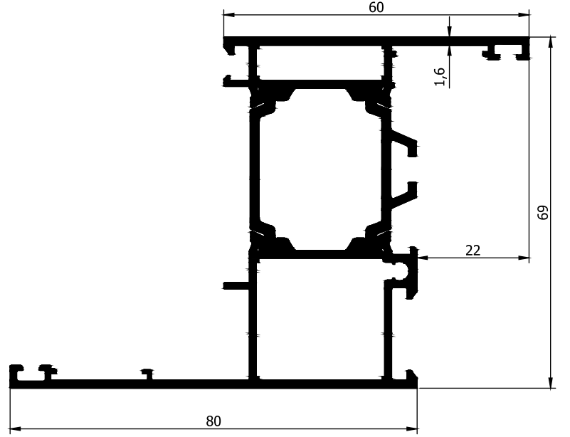
AD32-006 1,614 Kg/m
