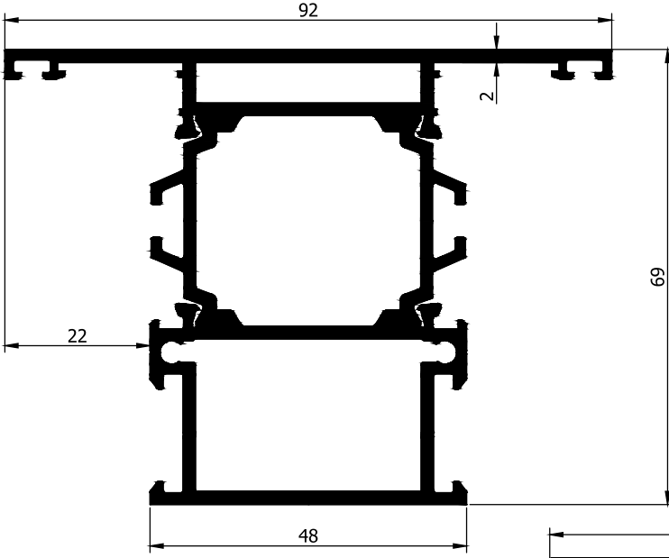
AD32-034 2,029 Kg/m
