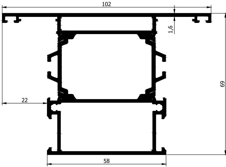
AD32-016 1,551 Kg/m
