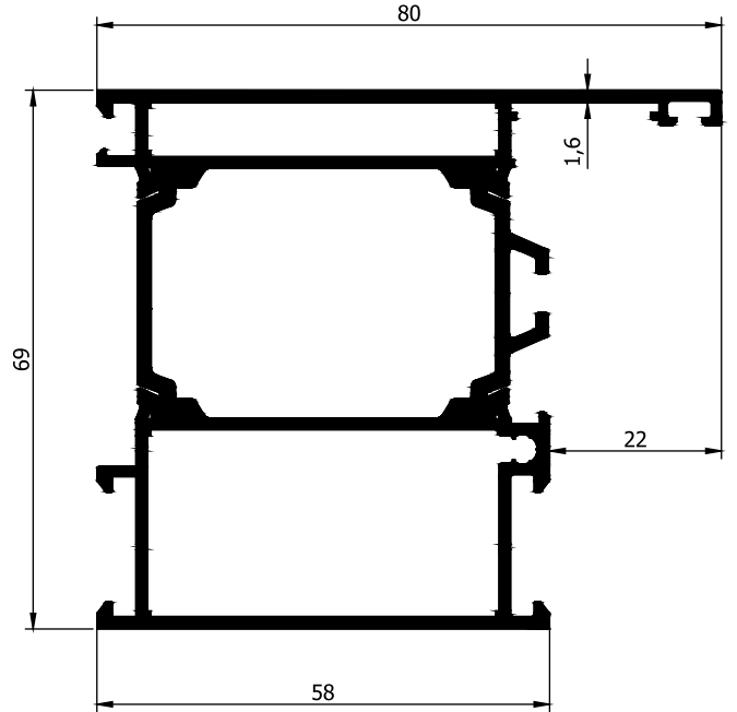
AD32-004 1,769 Kg/m
