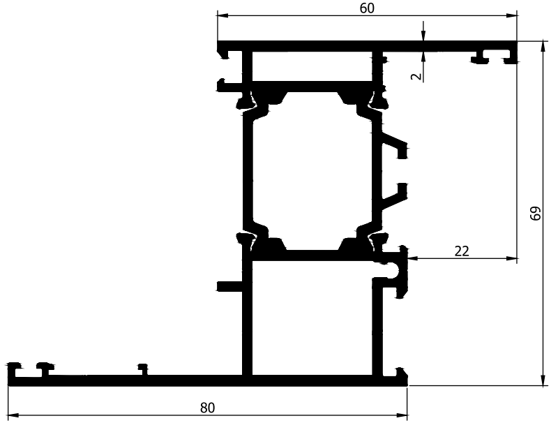
AD32-039 1,886 Kg/m
