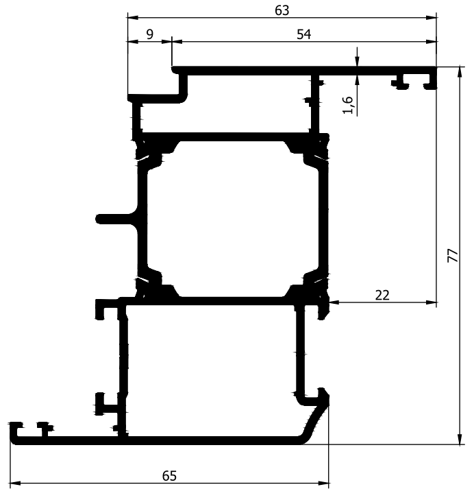
AD32-010 1,720 Kg/m
