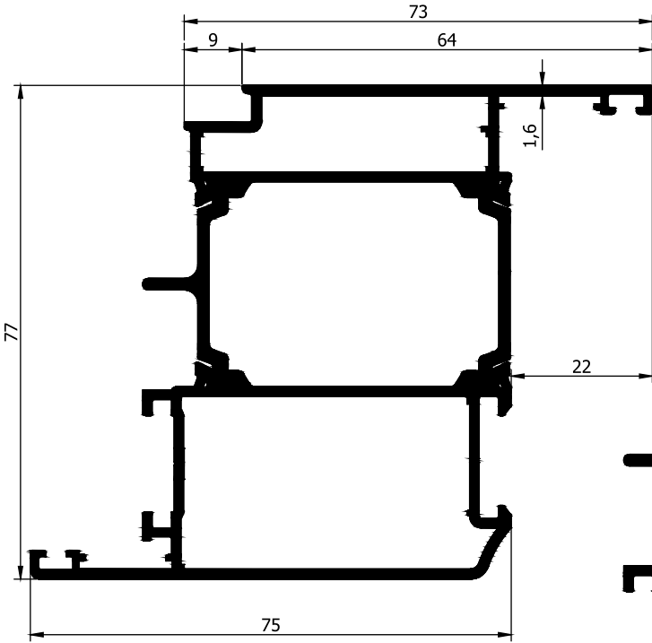
AD32-011 1,888 Kg/m
