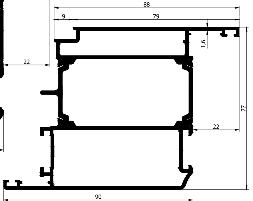
AD32-012 2,139 Kg/m
