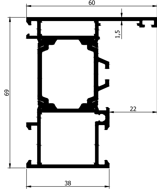
AD32-002 1,397 Kg/m
