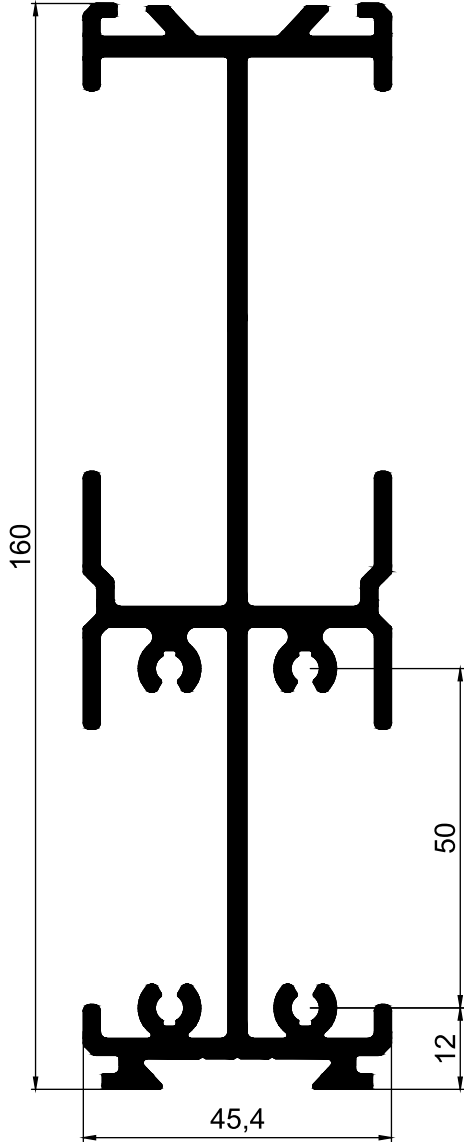
AD 22 - 062 ( 3,599 Kg/m )
