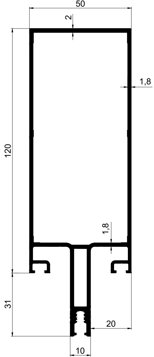
AD 22 - 004 ( 2,267 Kg/m )
