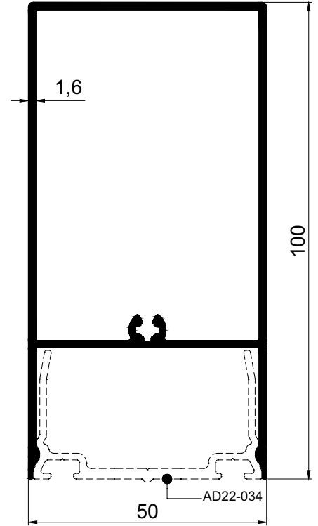
AD 22 - 035 ( 1,328 Kg/m )
