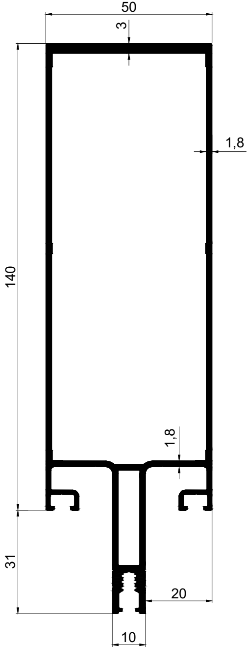
AD 22 - 005 ( 2,586 Kg/m )
