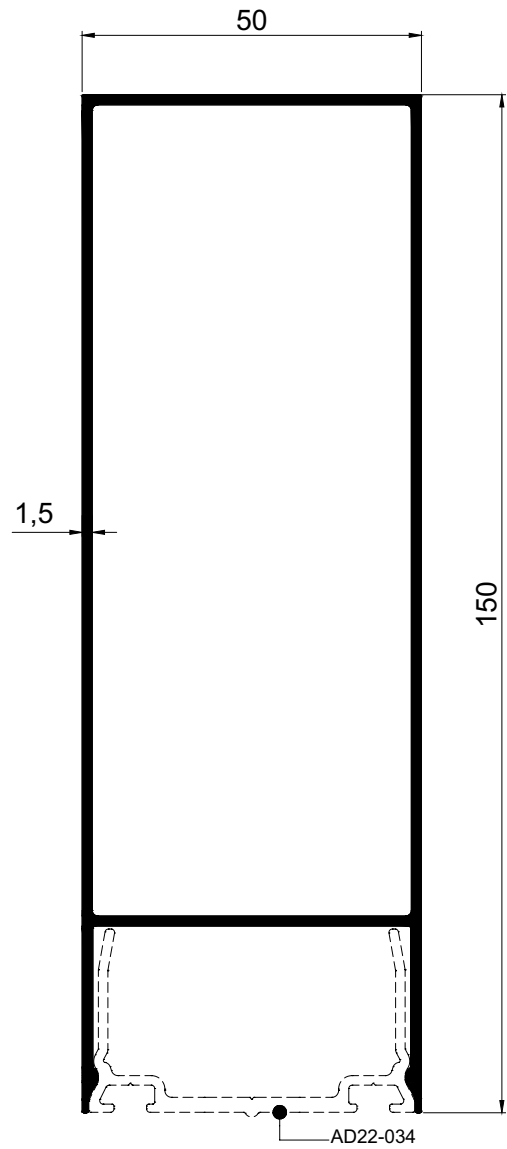
AD 22 - 092 ( 1,618 Kg/m )
