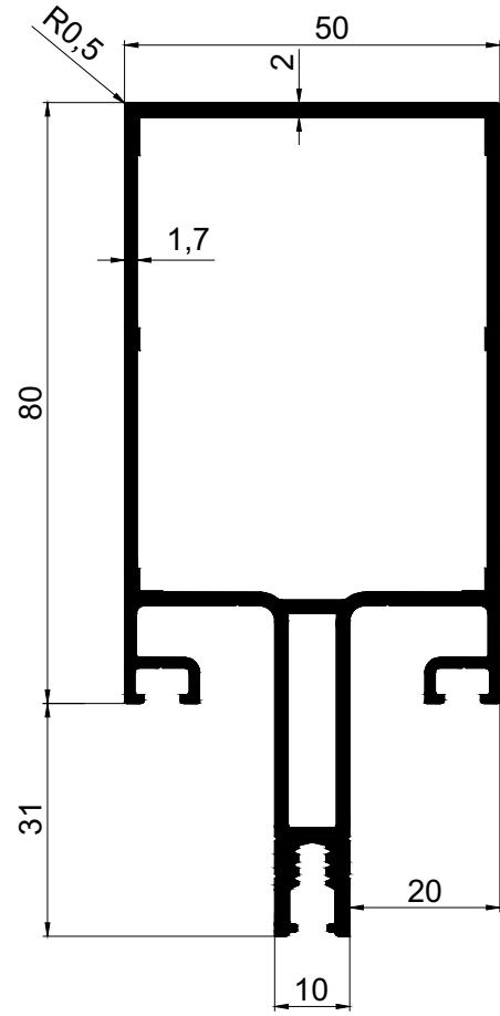
AD 22 - 002 ( 1,848 Kg/m )
